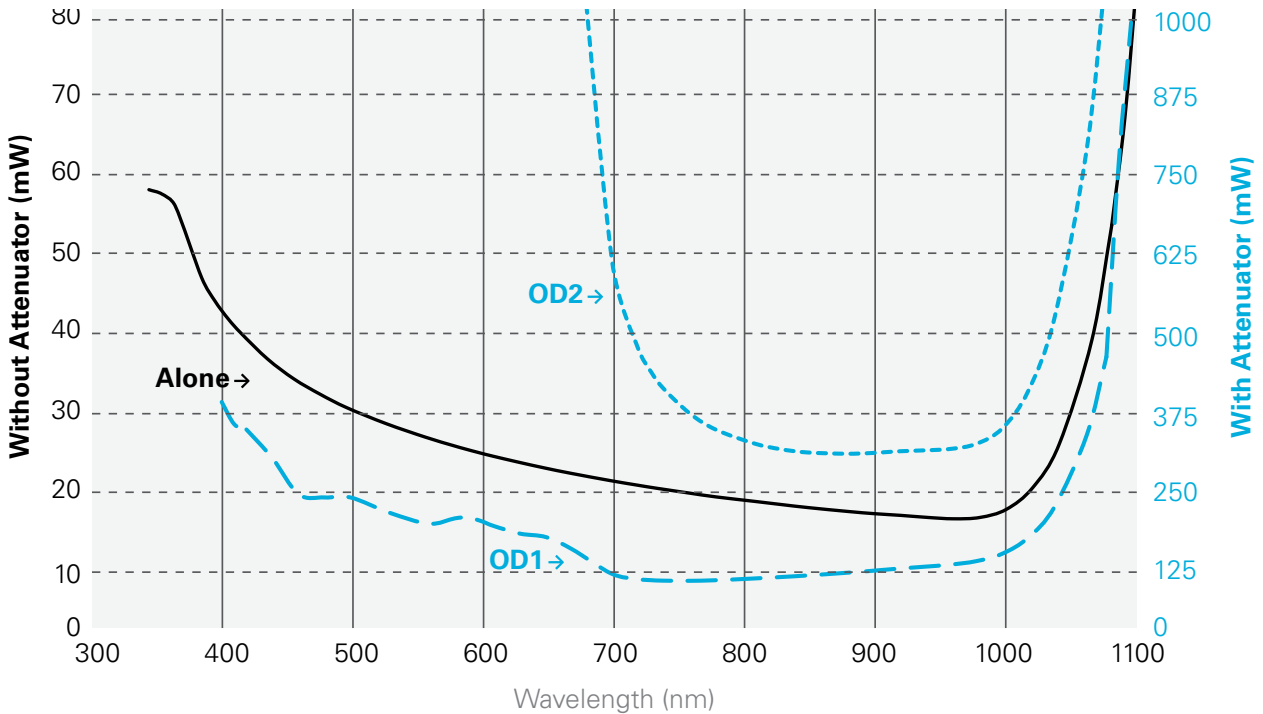
PH100-Si-HA Maximum Power
